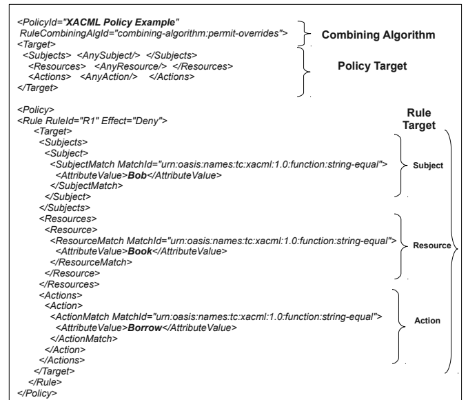
Figure 3: XACML Policy Example
